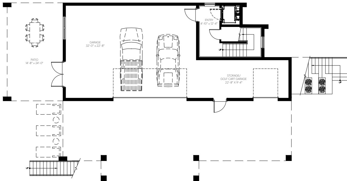
GROUND FLOOR
