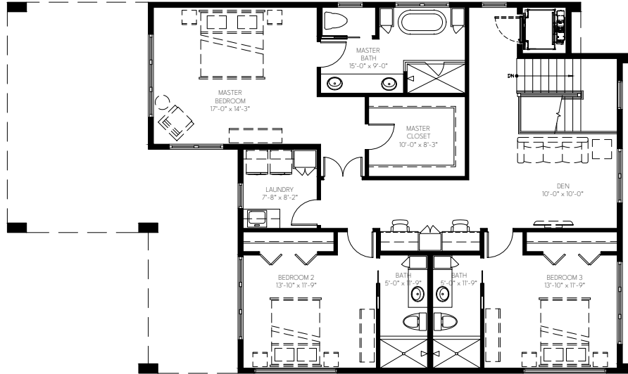
THIRD FLOOR
